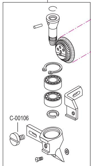
C-00081 C-00081G (versione rotella in gomma) (version with rubber roller foot)
