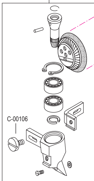
C-01058 C-01058G (versione rotella in gomma) (version with rubber roller foot)
