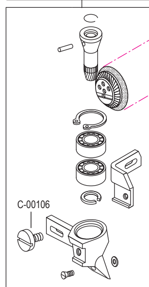
C-00081 C-00081G (versione rotella in gomma) (version with rubber roller foot)
